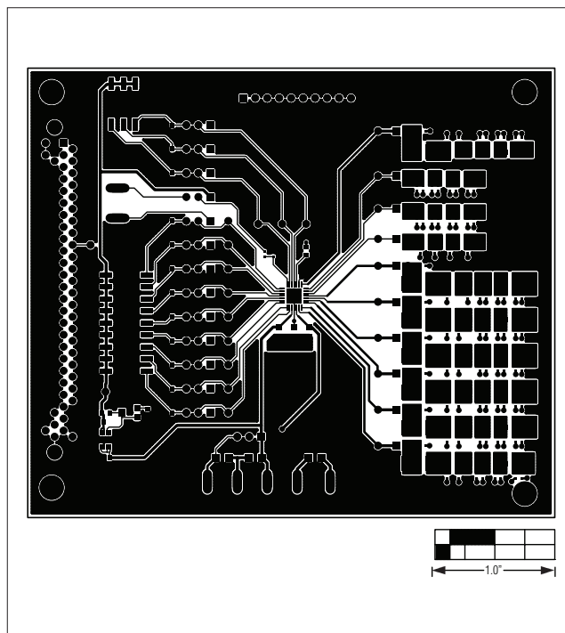
Figure 3. MAX17119 EV Kit PCB Layout—Component Side
