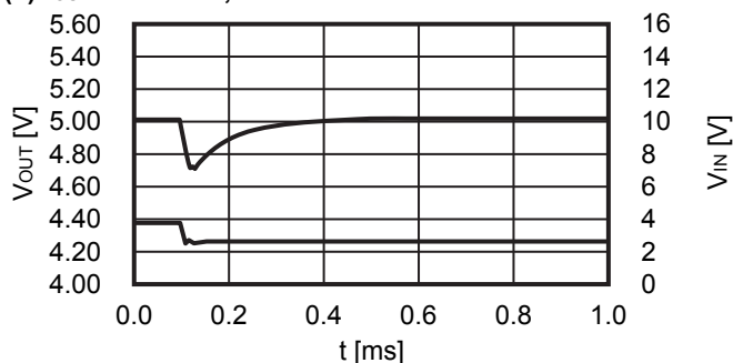
(4) f_{osc} = 600\text{ kHz} , V_{IN} = 3.8\text{ V} \rightarrow 2.8\text{ V} S-8366ABBBA
