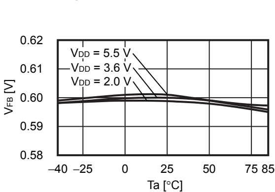
(11) FB voltage ( V_{FB} ) vs. Temperature ( T_a )
