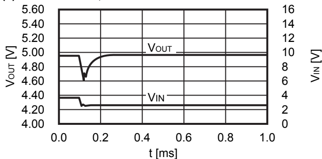
(2) f_{osc} = 1.2\text{ MHz} , V_{IN} = 3.8\text{ V} \rightarrow 2.8\text{ V} S-8366AABBA
