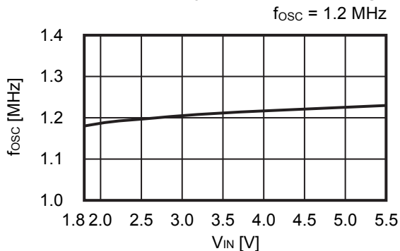
(3) Oscillation frequency ( f_{osc} ) vs. Input voltage ( V_{IN} )
