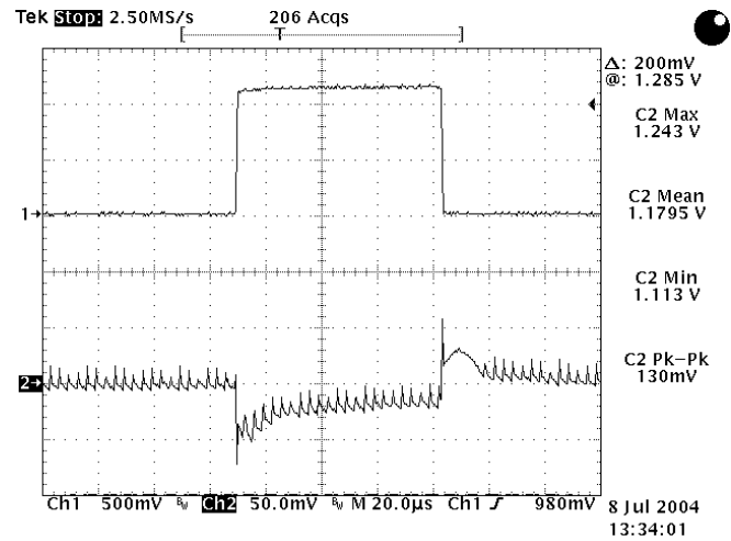
Figure 20: Typical transient response to step load change at 10\text{A}/\mu\text{S} from 50% to 75% and 75% to 50% of I_{o\_max} at 12\text{V}_{in} , 1.2V out
