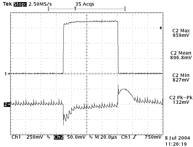
Figure 19: Typical transient response to step load change at 10\text{A}/\mu\text{S} from 50% to 75% and 75% to 50% of I_{o\_max} at 12\text{V}_{in} , 0.9V out
