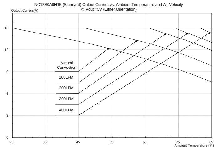
Figure 40: Output current vs. ambient temperature and air velocity @ Vout=5V(Either Orientation)
