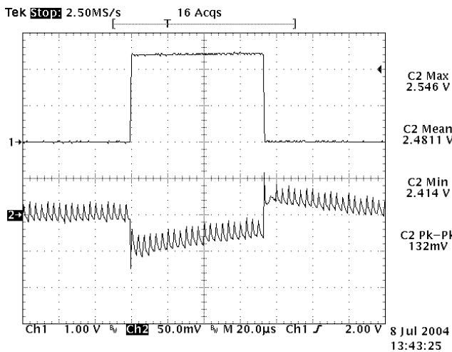
Figure 21: Typical transient response to step load change at 10\text{A}/\mu\text{S} from 50% to 75% and 75% to 50% of I_{o\_max} at 12\text{V}_{in} , 2.5V out
