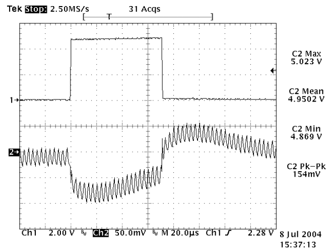
Figure 22: Typical transient response to step load change at 10\text{A}/\mu\text{S} from 50% to 75% and 75% to 50% of I_{o\_max} at 12\text{V}_{in} , 5.0V out
