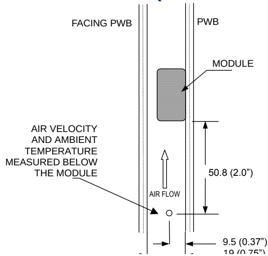
Figure 38: Wind tunnel test setup
