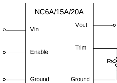
Figure 27: Trimming Output Voltage
