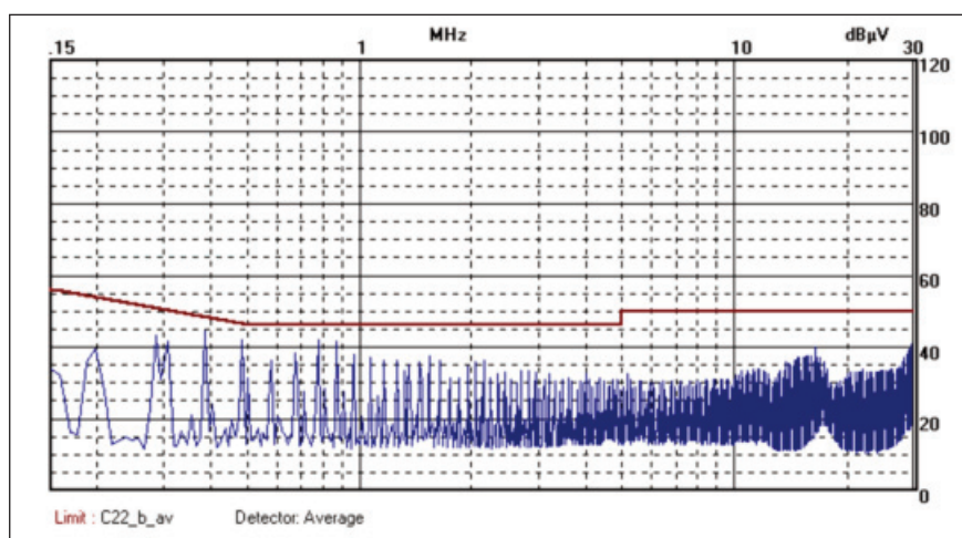
Figure 19 Typical EMC plot
