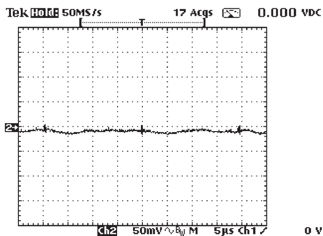
Figure 14 V3 (Full load). < 25 mV pk-pk Ripple. 20 MHz BW
