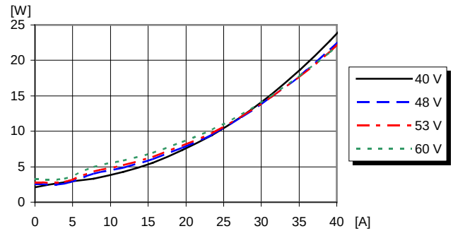
Dissipated power vs. load current and input voltage at T_{P1}, T_{P3} = +25^{\circ}\text{C}
