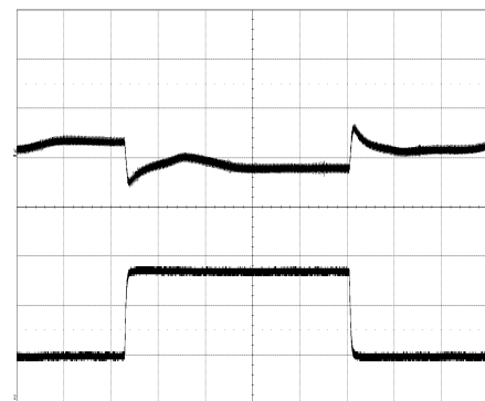
Output voltage response to load current step-change (17.5-52.5-17.5 A) at: T_{P1}, T_{P3} = +25^{\circ}\text{C}, V_i = 53 \text{ V}, C_O = 3.9 \text{ mF} Top trace: output voltage (0.5 V/div.). Bottom trace: output current (20 A/div.). Time scale: (0.5 ms/div.).
