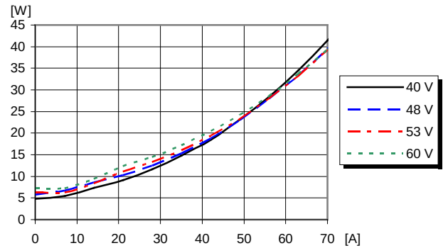
Dissipated power vs. load current and input voltage at T_{P1}, T_{P3} = +25^{\circ}\text{C}
