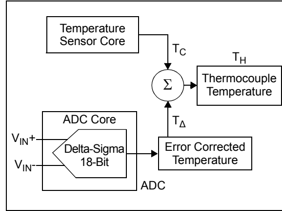
FIGURE 5-2: Thermocouple Temperature Register Block Diagram.
