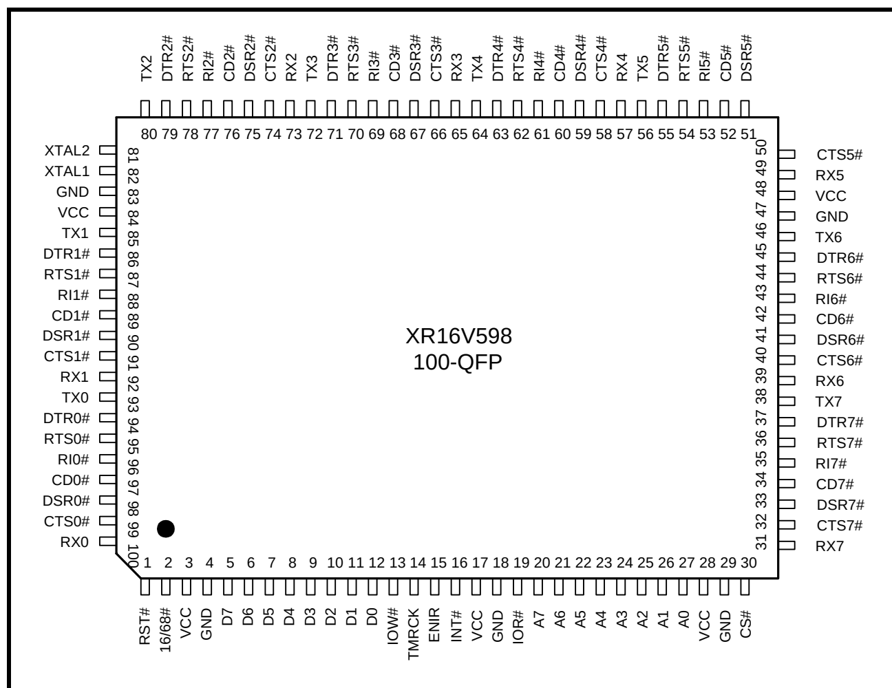
FIGURE 2. PIN OUT OF THE DEVICE
