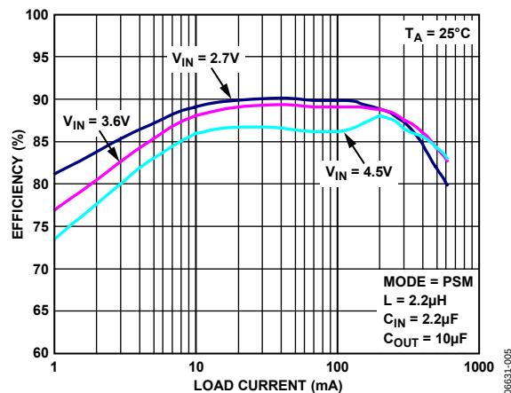
Figure 5. Efficiency vs. Load Current ( V_{OUT} = 1.5\text{ V} )
