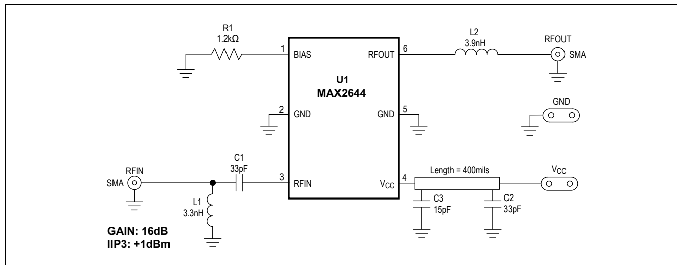
Figure 2. High Linearity Design
