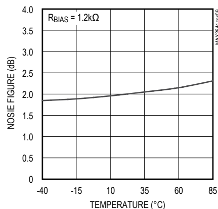
NOISE FIGURE vs. TEMPERATURE
