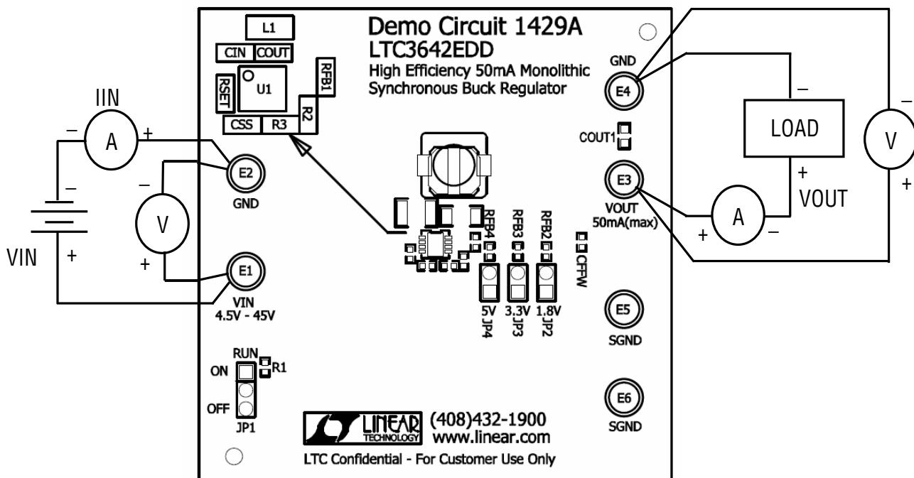
Figure 2. Equipment setup to test LTC3642
