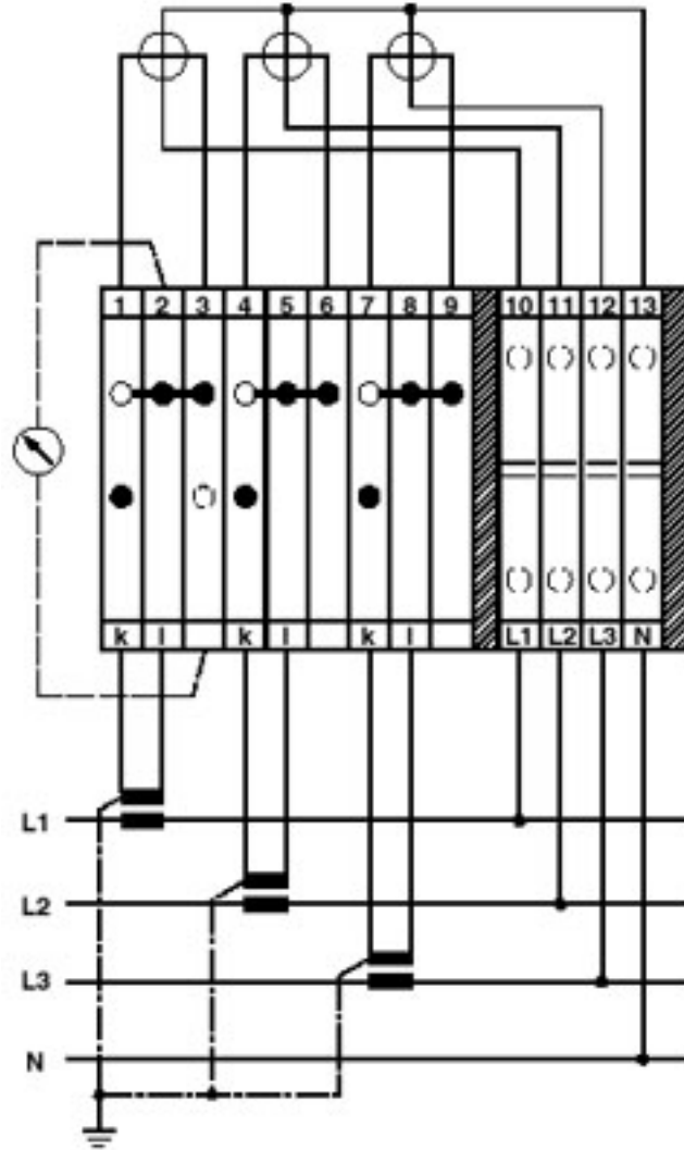
Meter test set (active current) constructed with UGSK and URTK-BEN
