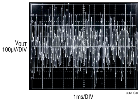
5V 10Hz to 100kHz Output Noise C_{\text{REF/BYP}} = 10\text{nF} , C_{\text{FF}} = 0
