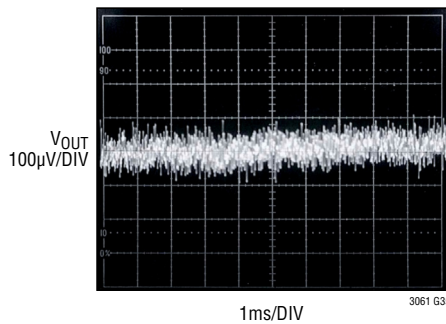
5V 10Hz to 100kHz Output Noise C_{\text{REF/BYP}} = 10\text{nF} , C_{\text{FF}} = 10\text{nF}
