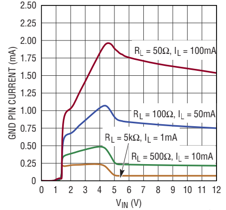
LT3061–5 GND Pin Current
