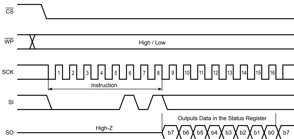
Figure 13 RDSR Operation
