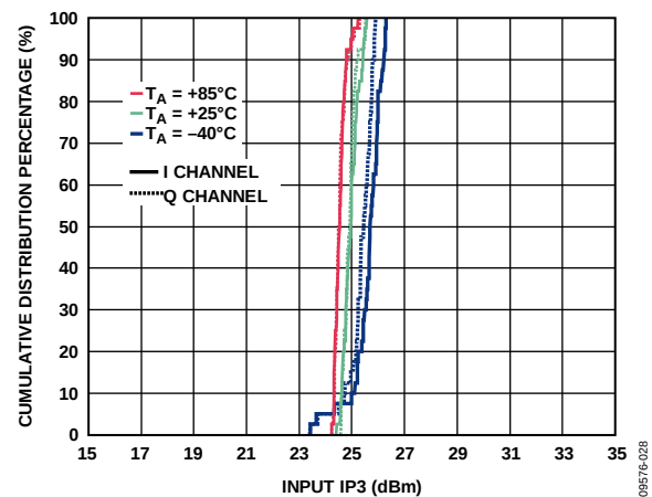
Figure 28. Input IP3
