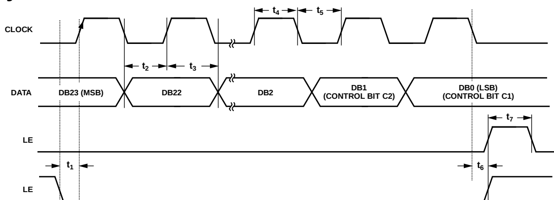
Figure 2. Timing Diagram
