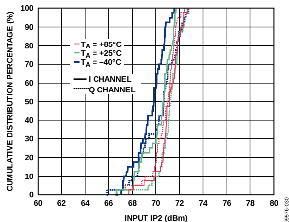
Figure 30. Input IP2
