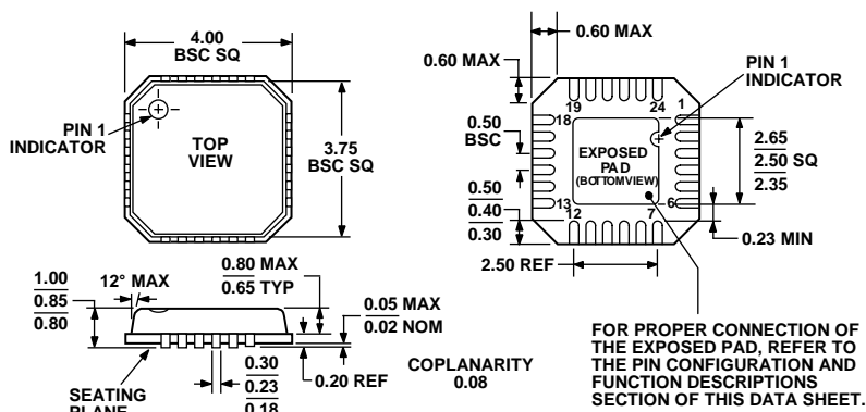
Figure 79. 24-Lead Lead Frame Chip Scale Package [LFCS_VQ] 4 mm × 4 mm Body, Very Thin Quad (CP-24-3) Dimensions shown in millimeters
