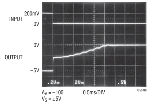
Overload Recovery
