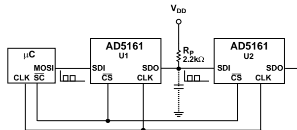
Figure 43. Daisy-Chain Configuration
