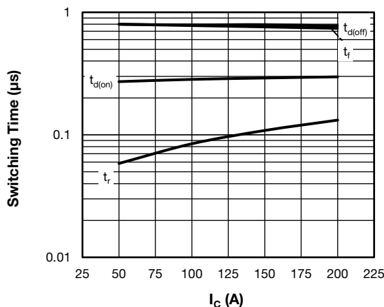
Fig. 10 - Typical IGBT Switching Time vs. I_C T_J = 125\text{ }^\circ\text{C} , V_{CC} = 480\text{ V} , V_{GE} = 15\text{ V} , L = 500\text{ }\mu\text{H} , R_g = 5\text{ }\Omega Diode used: 60APH06
