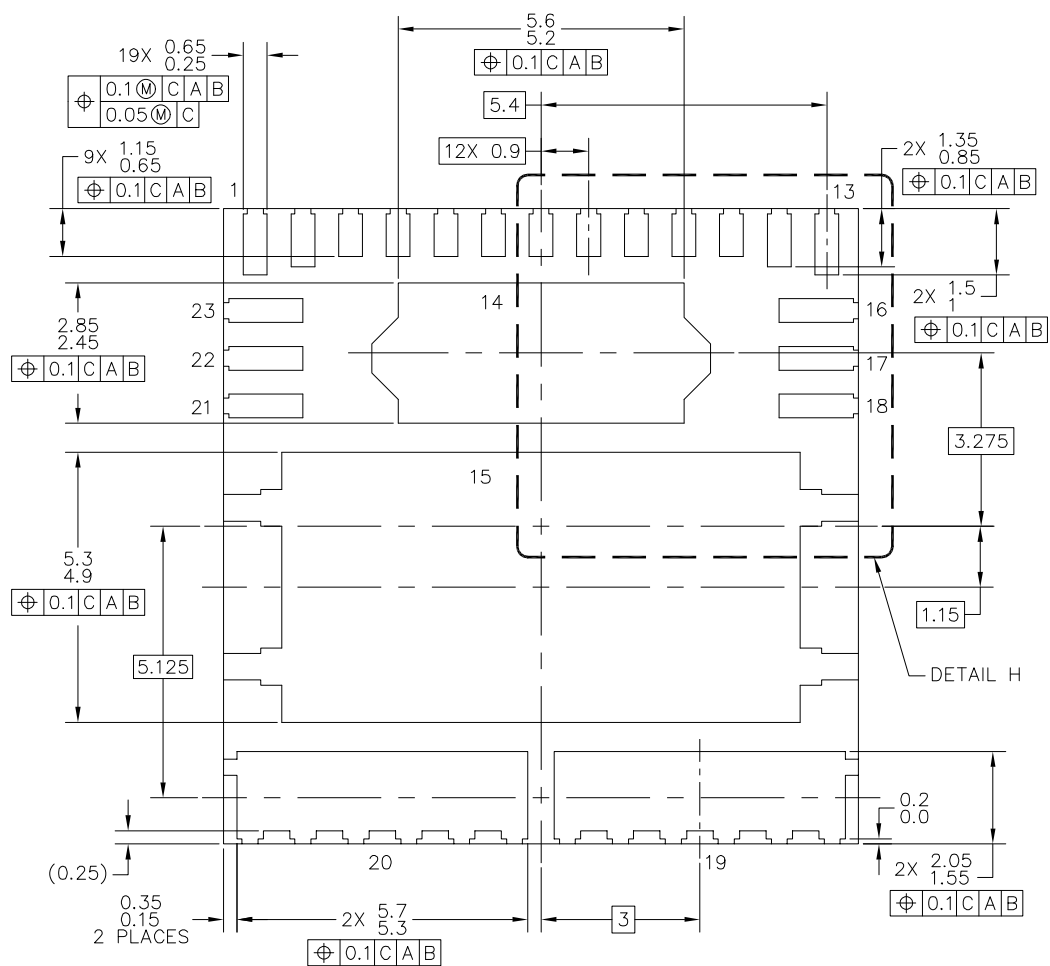
VIEW M-M
