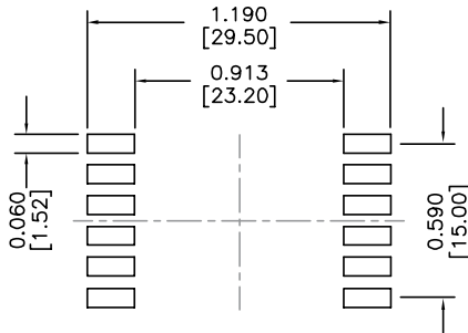
Recommended Footprint
