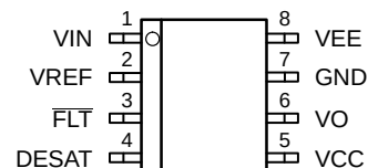
NCD5703B
