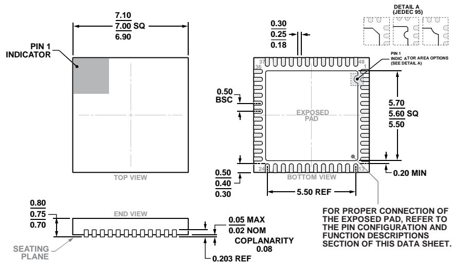
Figure 66. 48-Lead Lead Frame Chip Scale Package [LFCS] 7 mm × 7 mm Body and 0.75 mm Package Height (CP-48-13)
