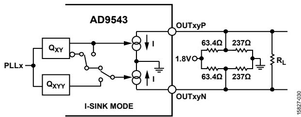
Figure 35. LVDS-Compatible Output, 1.2 V Common-Mode, Thevenin Bias Network ( I = 7.5 mA; 15 mA With Extra 100 Ω Termination, R_t )
