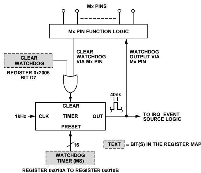
Figure 49. Watchdog Timer
