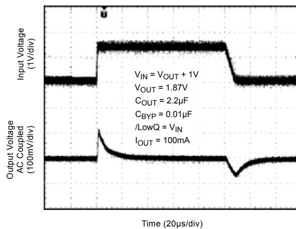
DC/DC Line Transient PWM Mode
