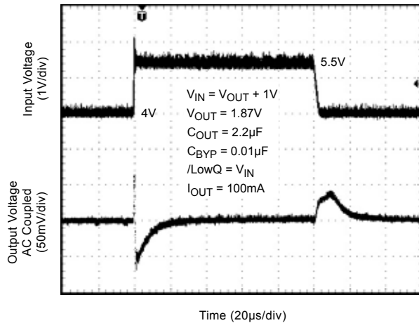
LDO2 Line Transient Normal Mode
