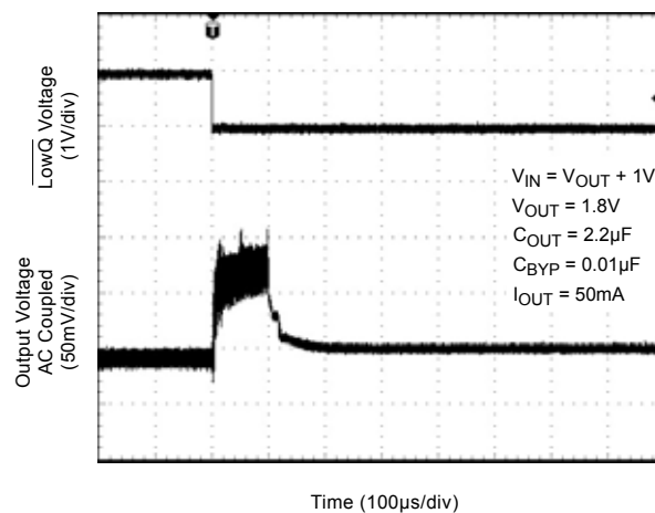
DC/DC PWM Mode to LowQ Mode Transition
