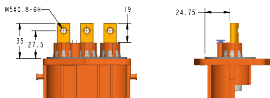
Busbar Type 1
