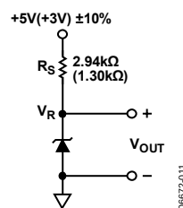
Figure 11. Typical Connection Diagram
