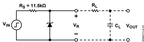
Figure 19. Turn-On, Settling, and Transient Test Circuit
