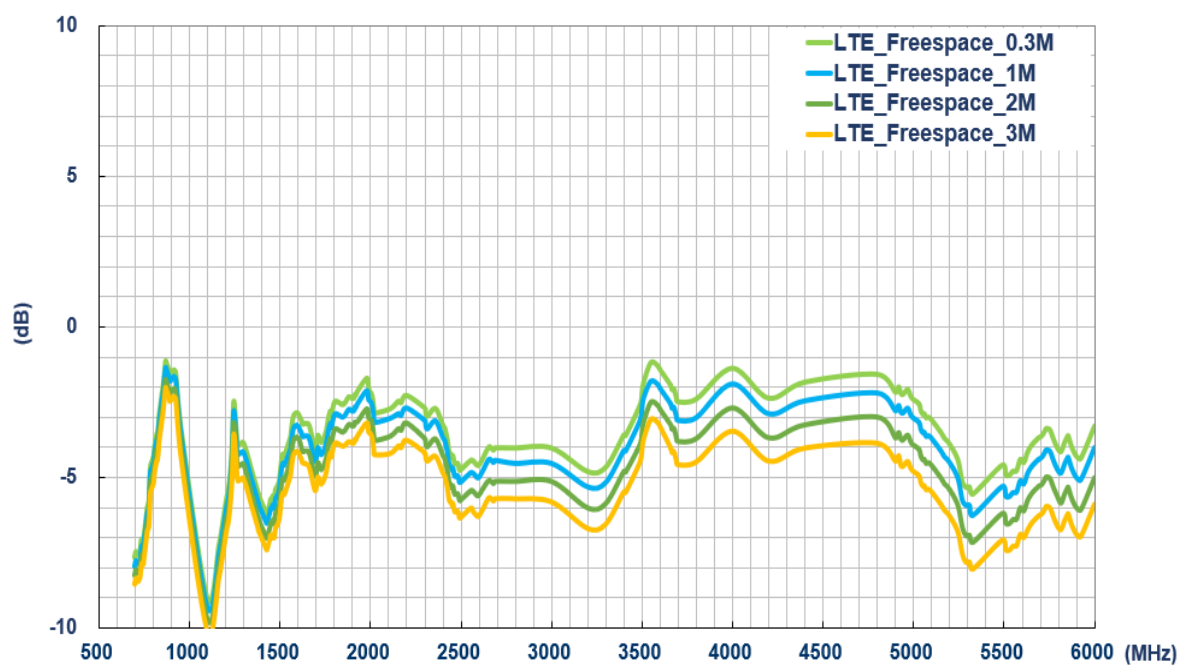
Average Gain – LTE Antenna (Free Space)
