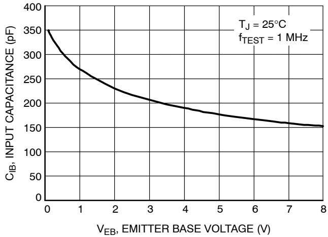
Figure 10. Input Capacitance
