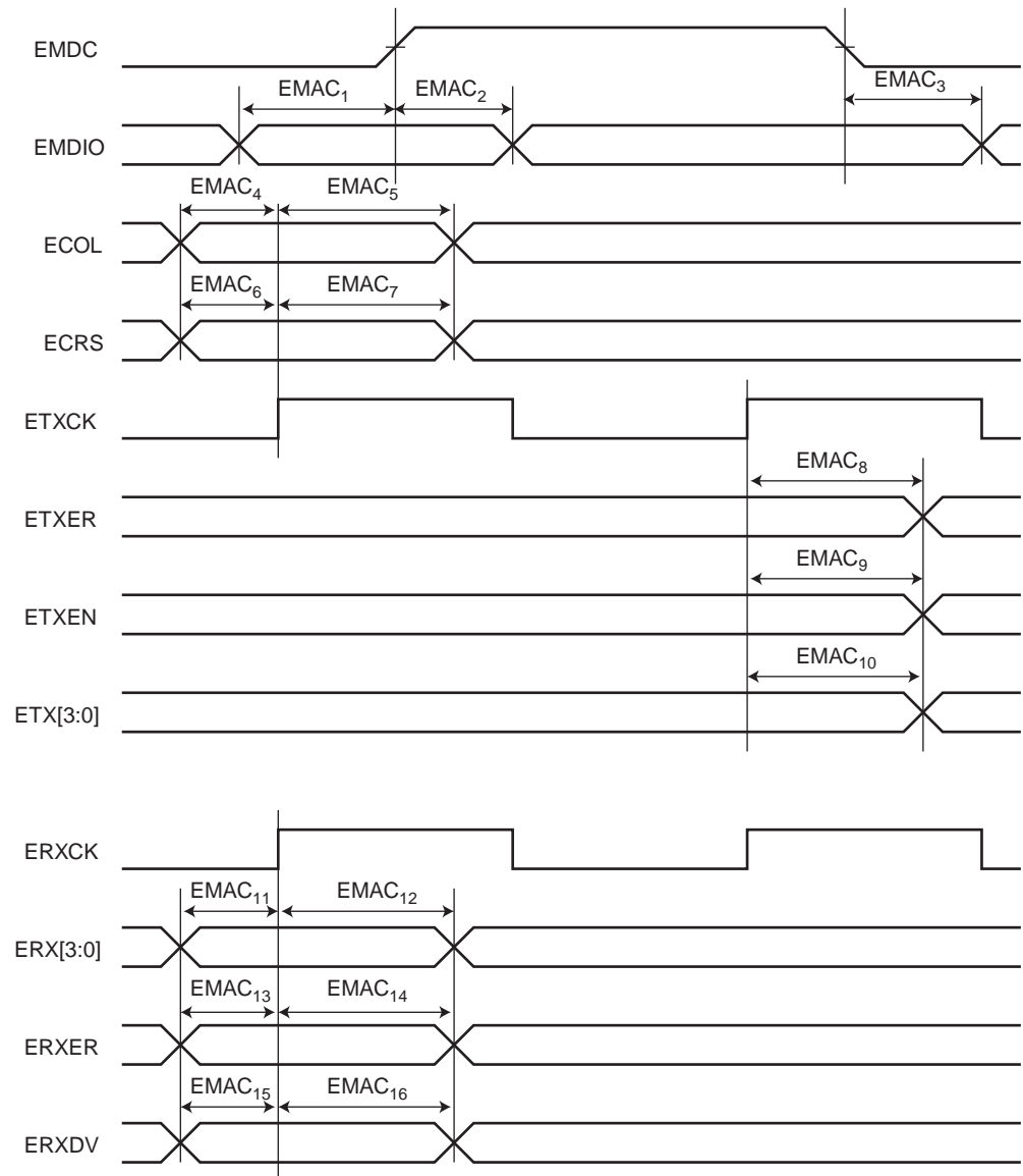
Figure 38-8. EMAC MII Mode
