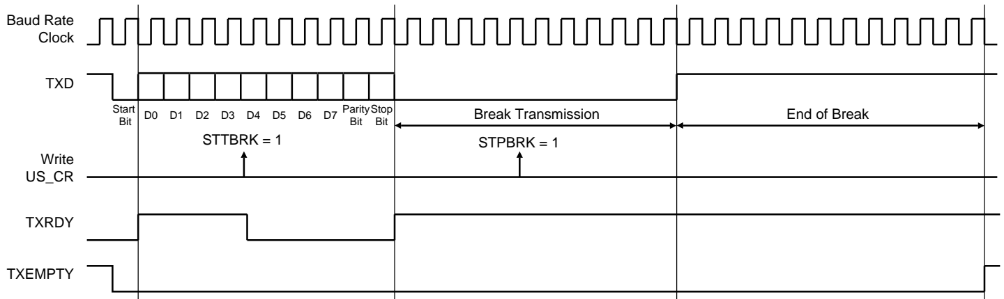
Figure 30-16. Break Transmission
