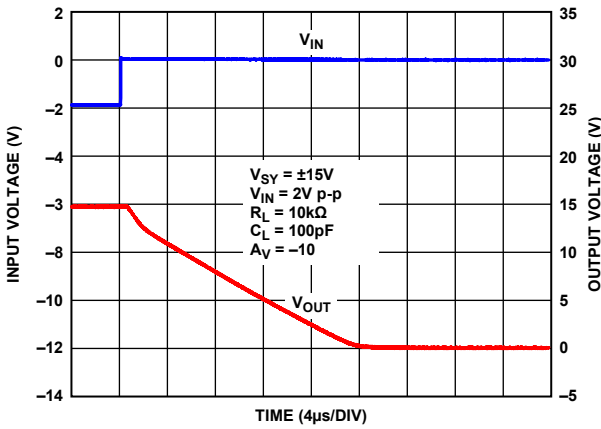
Figure 53. Positive Overload Recovery, V_{SY} = \pm 15\text{ V}
