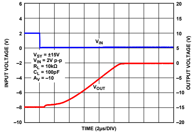
Figure 56. Negative Overload Recovery, V_{SY} = \pm 15\text{ V}
