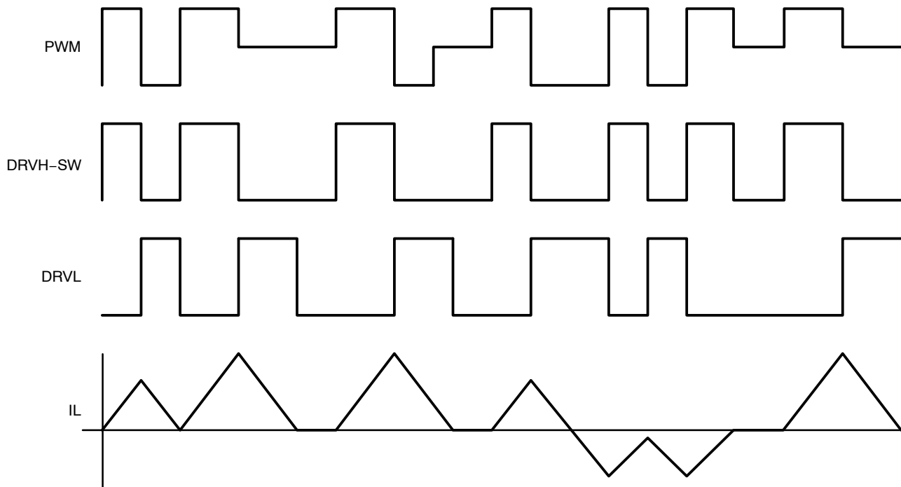
Figure 4. Timing Diagram
