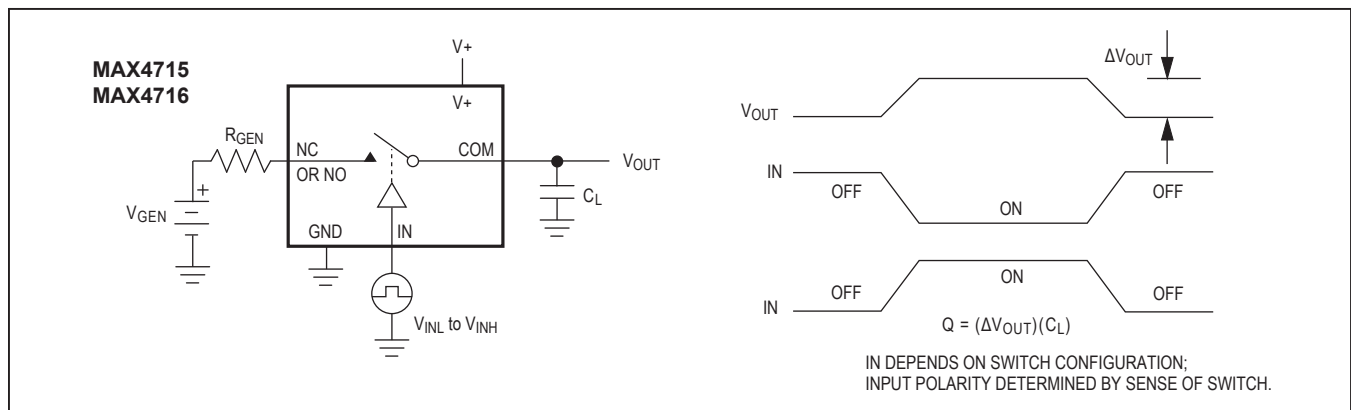
Figure 2. Charge Injection
