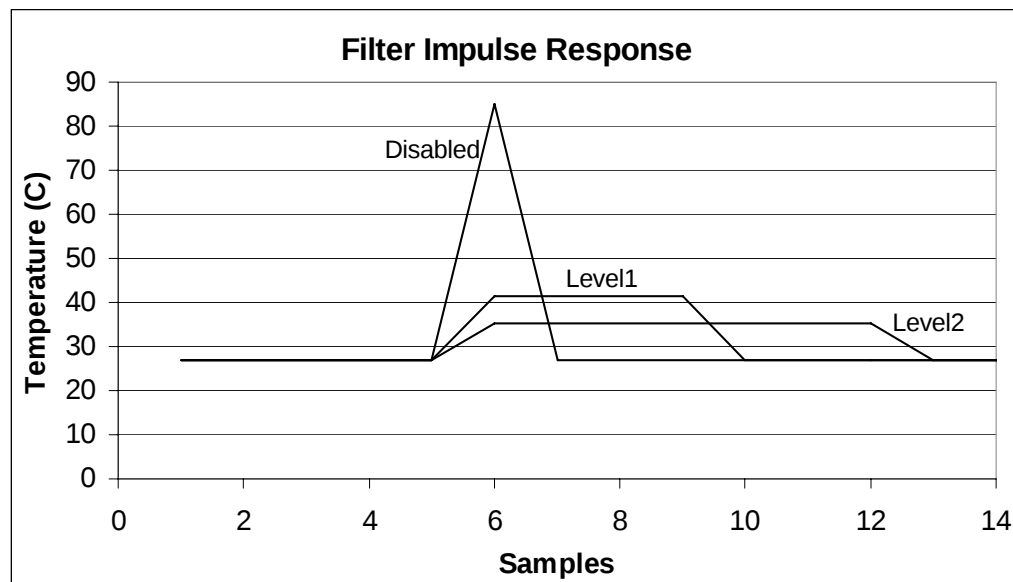
Figure 5.6 Temperature Filter Impulse Response
