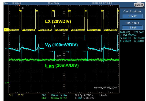
FIGURE 15. V_{OUT} RIPPAGE VOLTAGE
