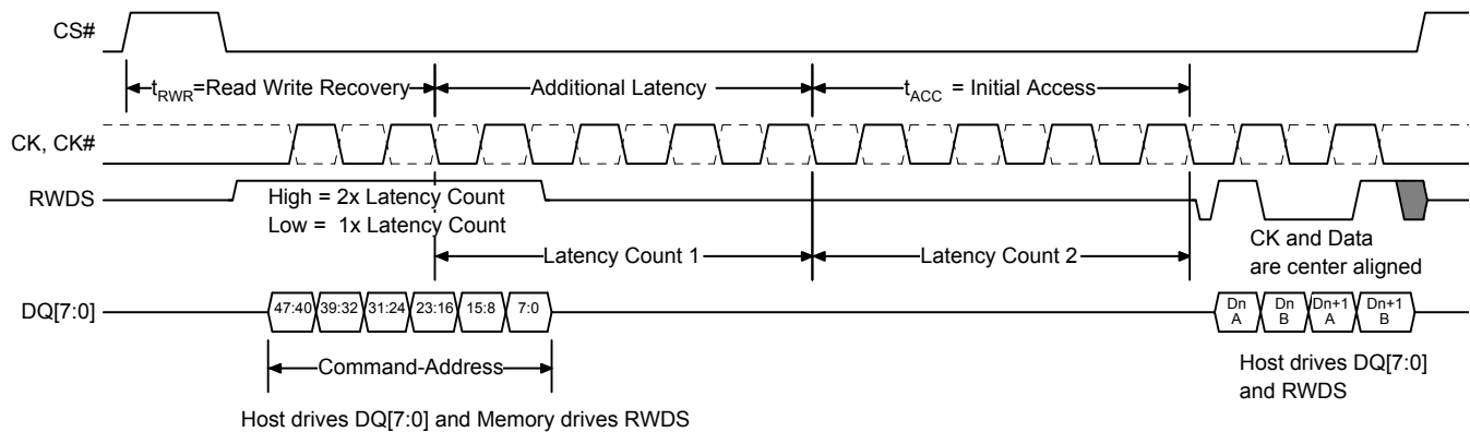
Figure 11.6 Write Transaction with Additional Initial Latency
