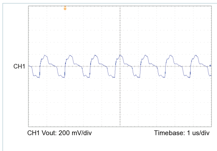
Figure 19 — Output voltage ripple, V_{IN} = 30\text{ V} , V_{OUT} = 28.0\text{ V} , C_{OUT\_EXT} = 1000\text{ }\mu\text{F} , R_{LOAD} = 4.828\text{ }\Omega
