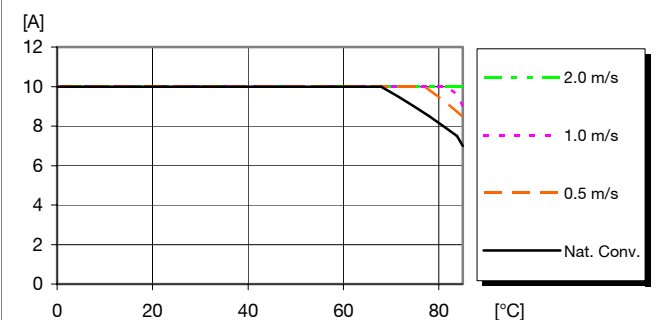
Available load current vs. ambient air temperature and airflow at V_I = 12.0\text{ V} , V_{OUT} = 5.0\text{ V} . See Thermal Consideration section.
