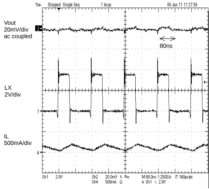
Figure 23. Fig.23 PWM mode Operation I_{out} = 100\text{mA}
