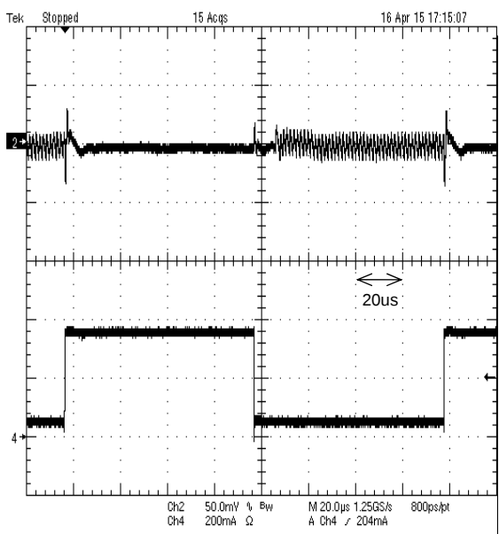
Figure 53. Load transient response 50mA to 350mA t_r=t_f=100\text{ns} , MODE : High
