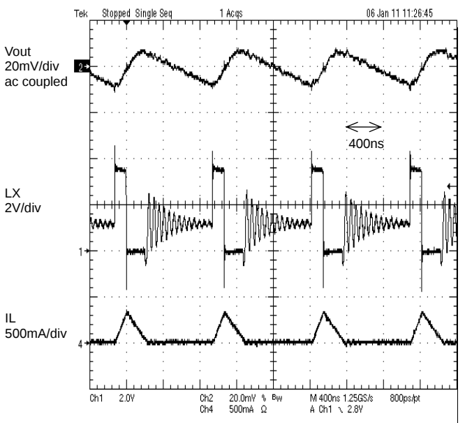
Figure 22. PFM mode Operation I_{out} = 50\text{mA}
