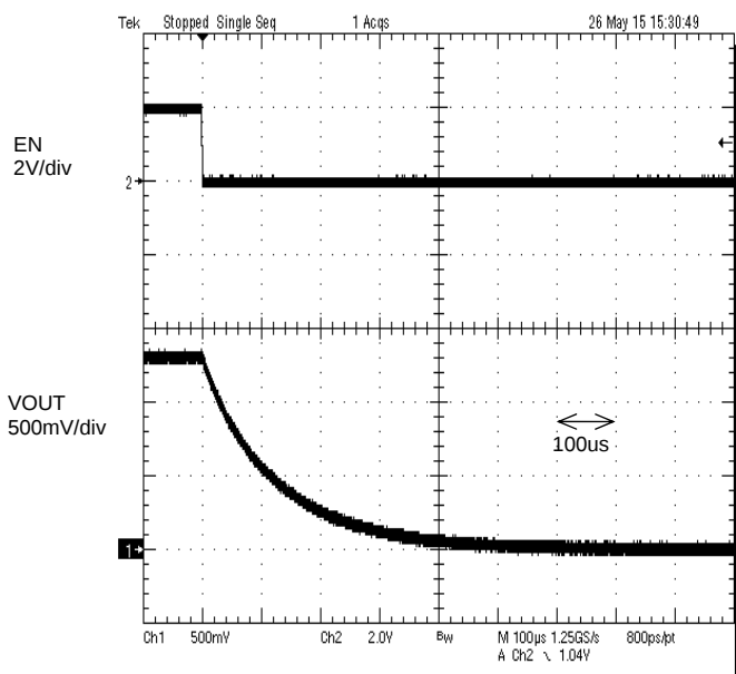
Figure 62. Shut down
