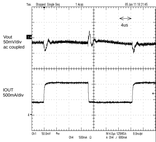
Figure 21. Load transient response 400mA to 1000mA t_r = 100\text{ns} , MODE : Low
