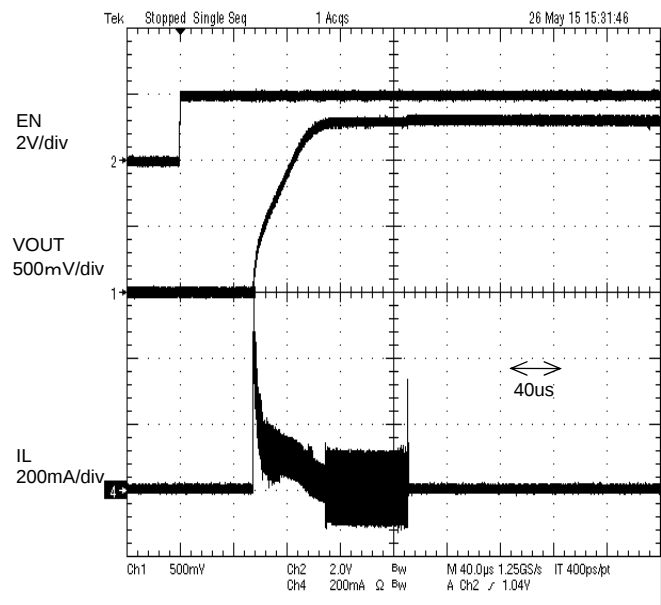
Figure 61. Start up
