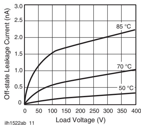
Fig. 12 - Leakage Current vs. Applied Voltage at Elevated Temperatures
