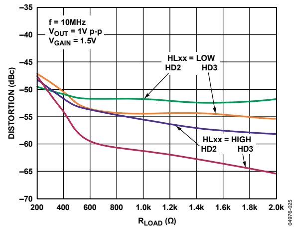
Figure 25. Harmonic Distortion vs. R_{\text{LOAD}} (See Figure 53)
