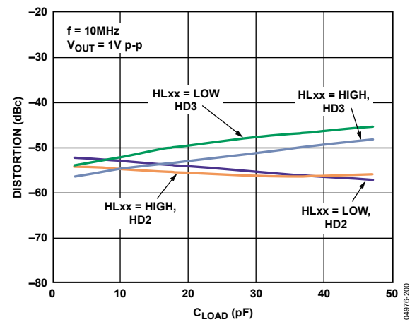
Figure 26. Harmonic Distortion vs. C_{\text{LOAD}} (See Figure 53)
