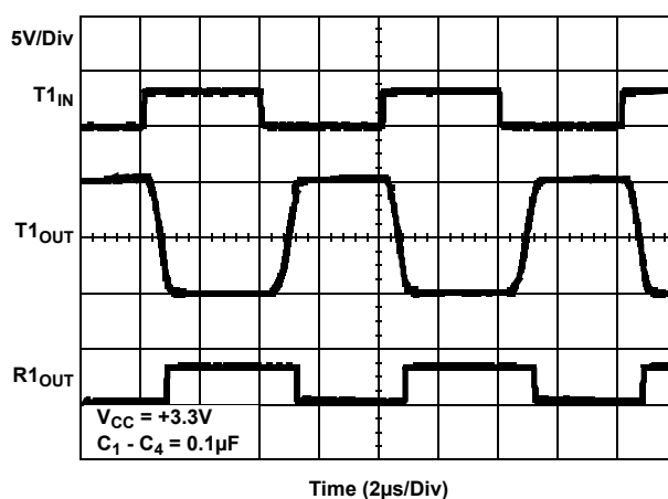
Figure 16. Loopback Test at 250kbps
