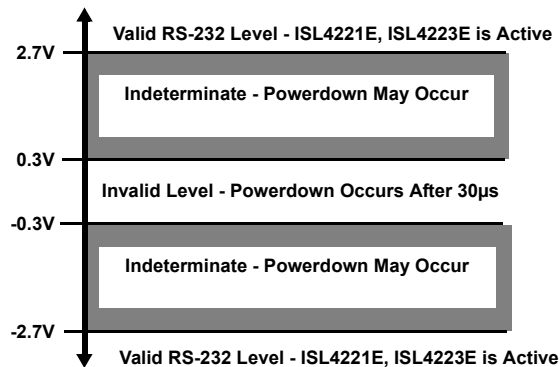
Figure 10. Definition of Valid RS-232 Receiver Levels
