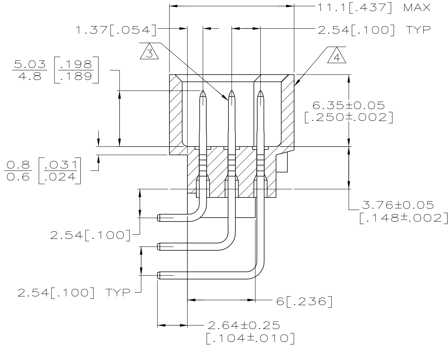
SECTION Z-Z
