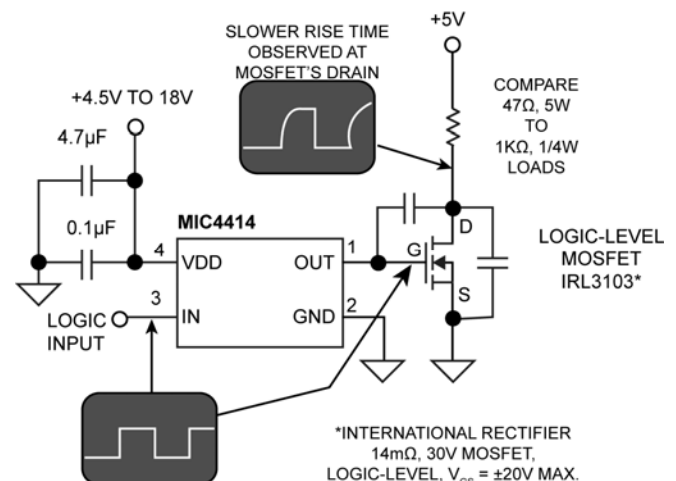
Figure 4. MOSFET Capacitance Effects at High Switching Frequency
