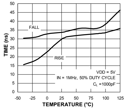
Rise and Fall Time vs. Temperature
