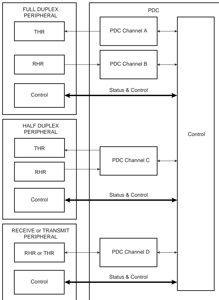
Figure 22-1. Block Diagram
