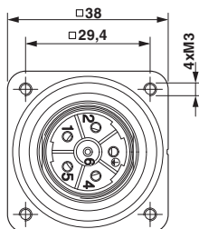
Flange dimensions
